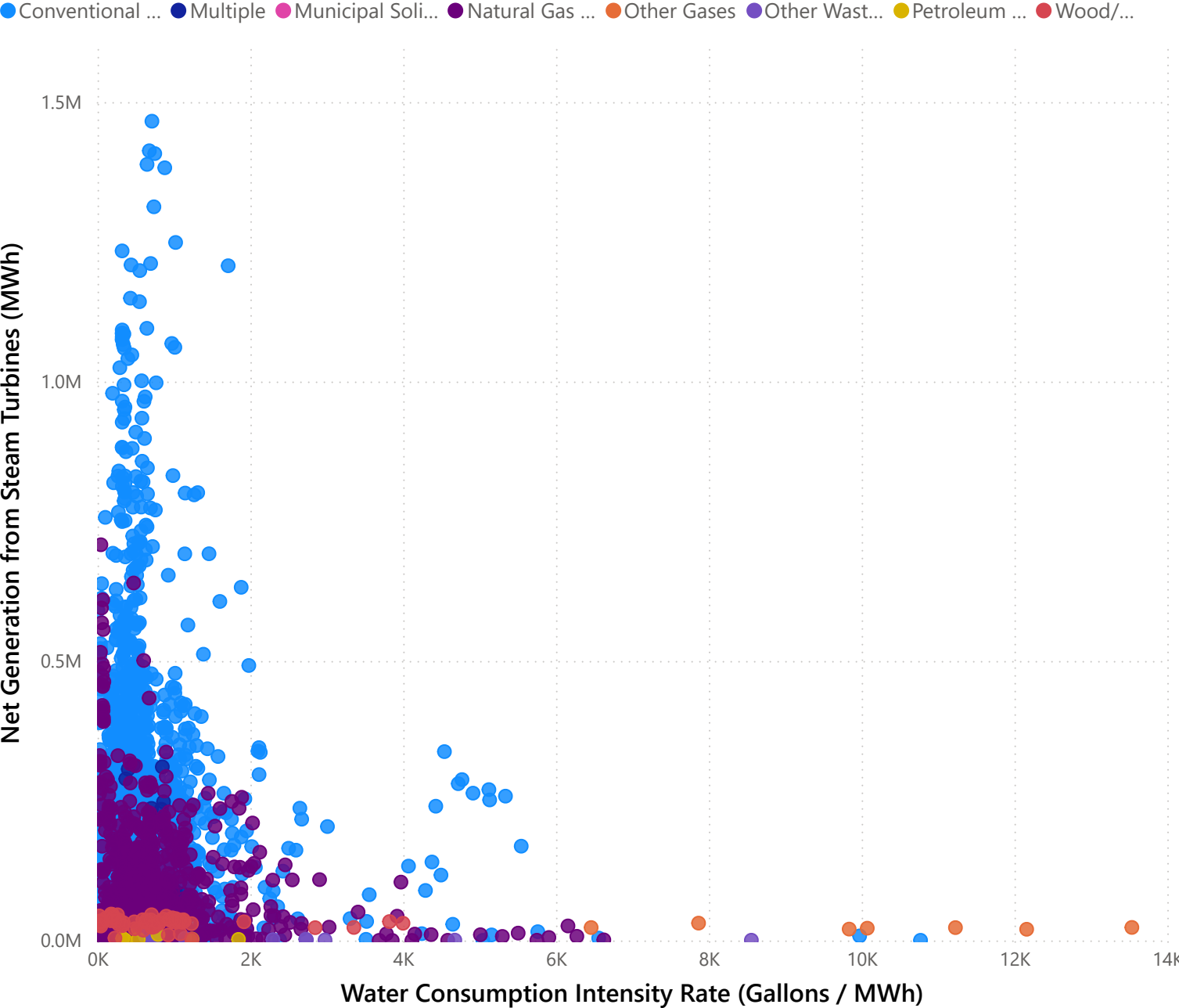
Generator Primary Technology, Water Consumption Intensity Rate (Gallons / MWh) and Net Generation from Steam Turbines (MWh)
